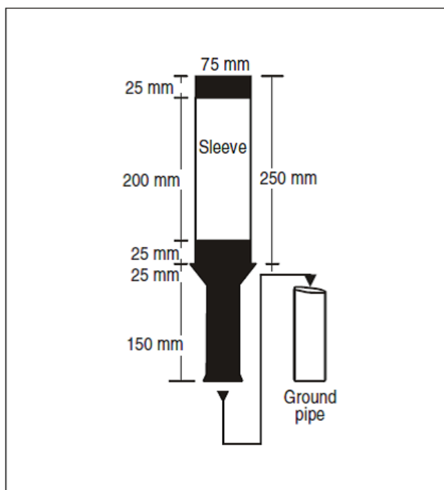
Figure GM-P-1. Taxiway edge marker
