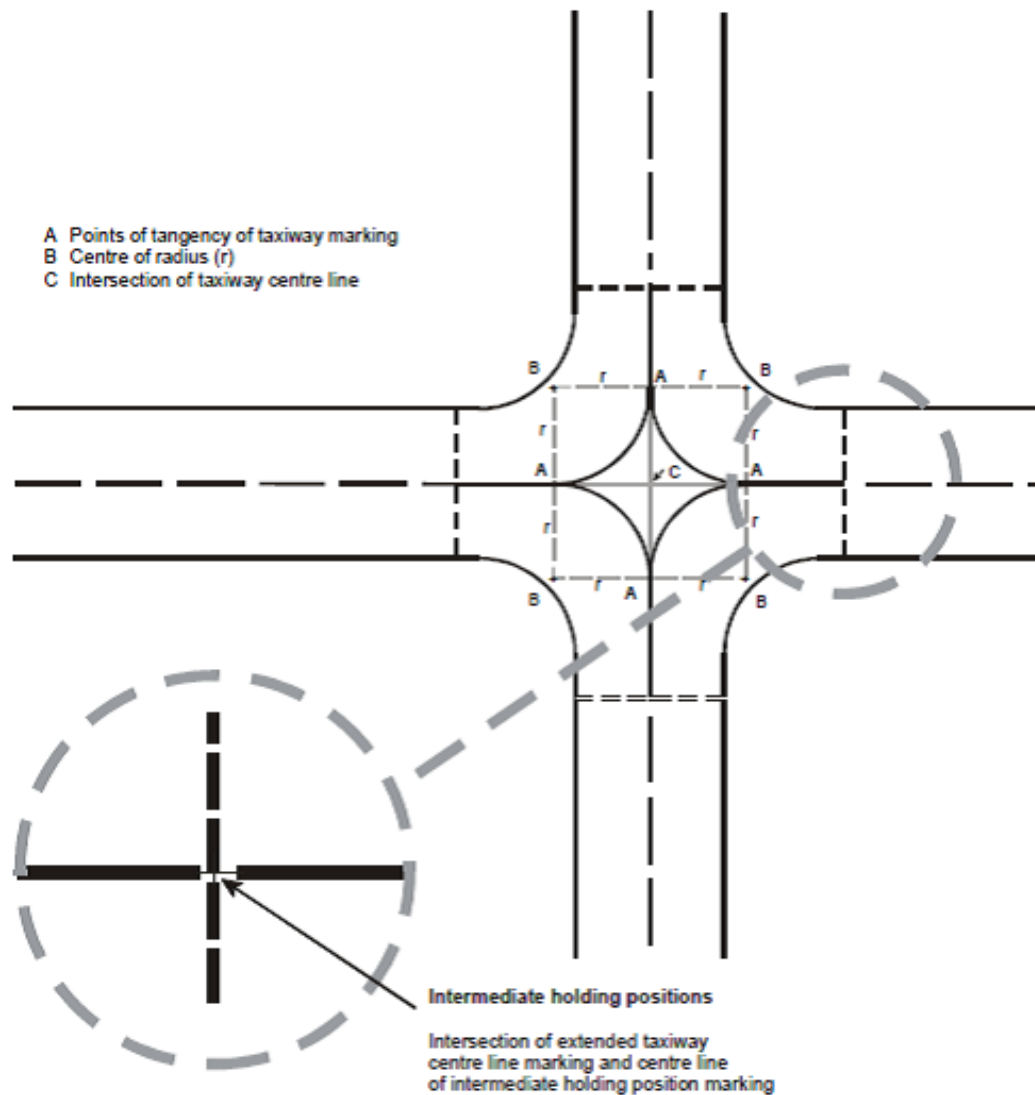
Figure 7 - Taxiway intersections to be surveyed
