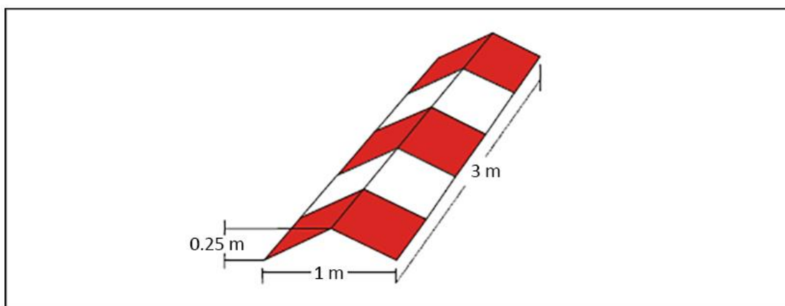
Figure GM1-F-1. Runway-type FATO edge marker
