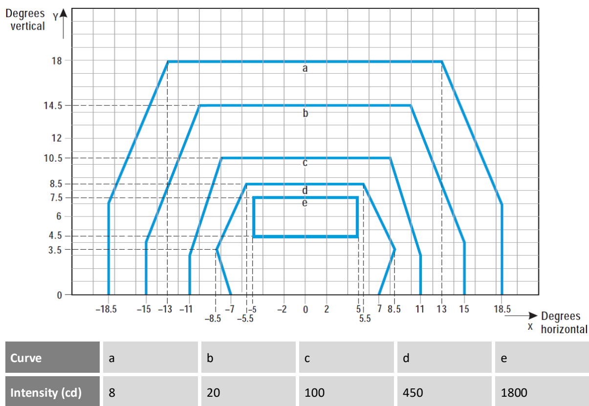
Figure U-22. Isocandela diagram for high-intensity taxiway centre line (15 m spacing), no-entry bar, and stop bar lights in straight sections intended for use in an advanced surface movement guidance and control system where higher light intensities are required
