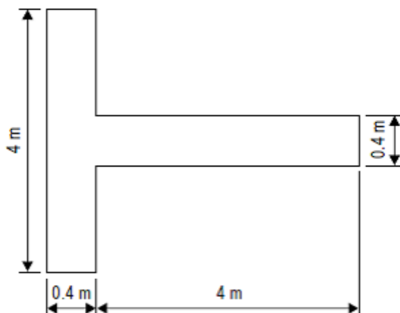
Figure K-1. Landing direction indicator
